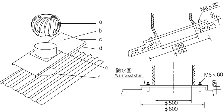
钢筋屋顶装设排风器示意图 The chart of installation on reinforced concrete roof 钢筋混凝土屋顶装设排风器 (20") 示意图 The chart of installation on reinforced concrete roof
