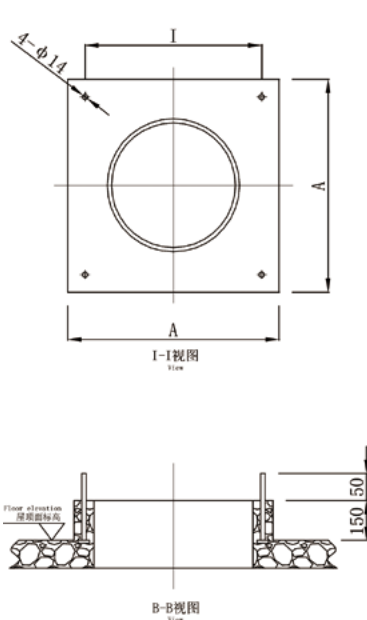
Performance and installation external dimensions of the BDW-87-3 power roof fan
